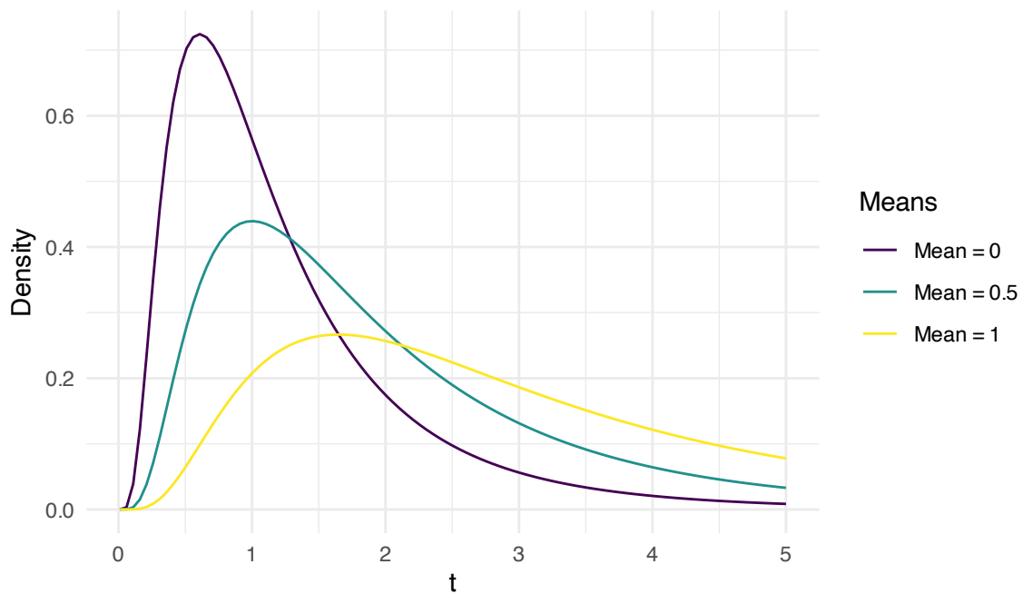
Lognormal Densities with Different Means
